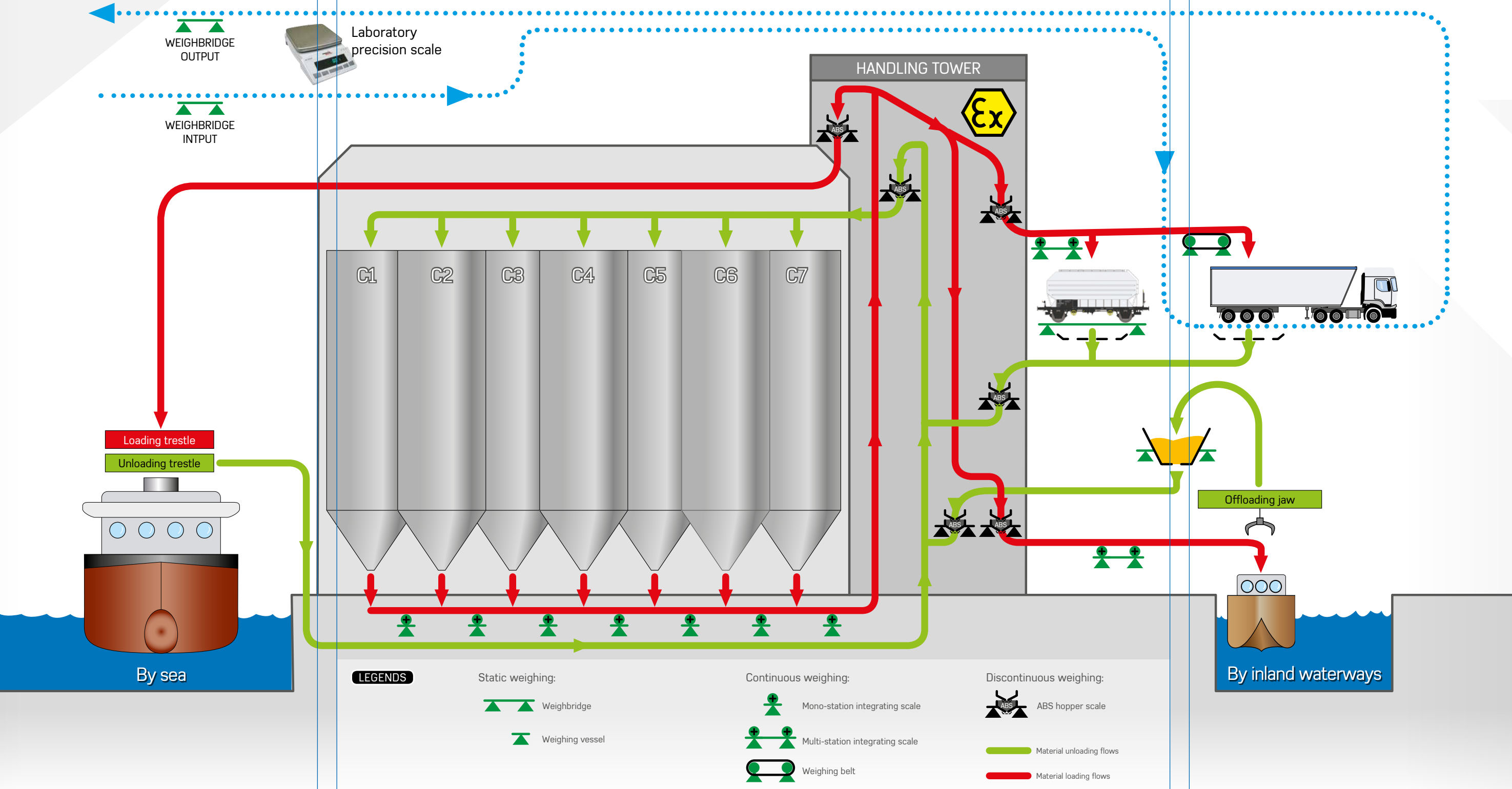
WEIGHBRIDGES HANDLING TRUCK INPUT/OUTPUT
