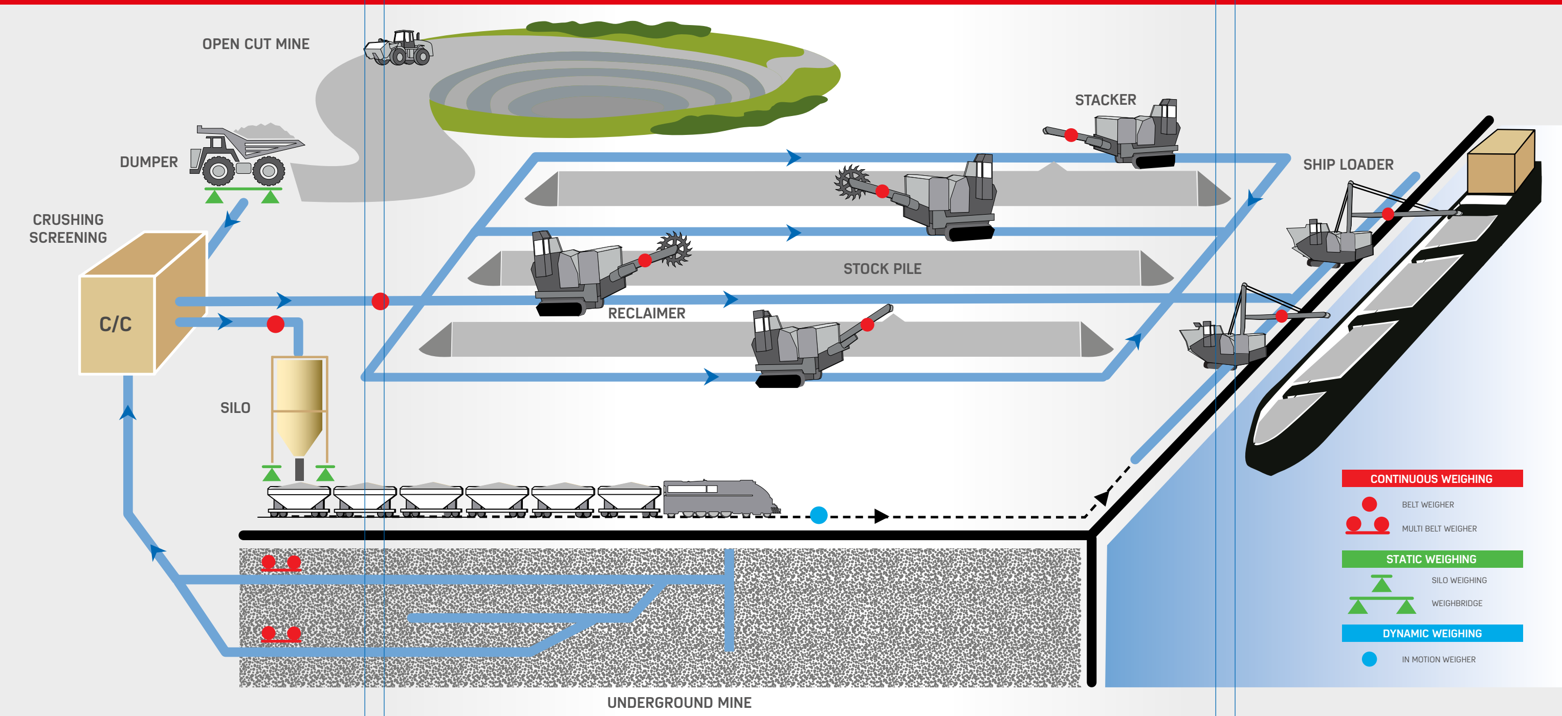
BELT WEIGHING
